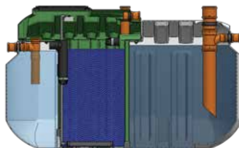
Reactor Zone
